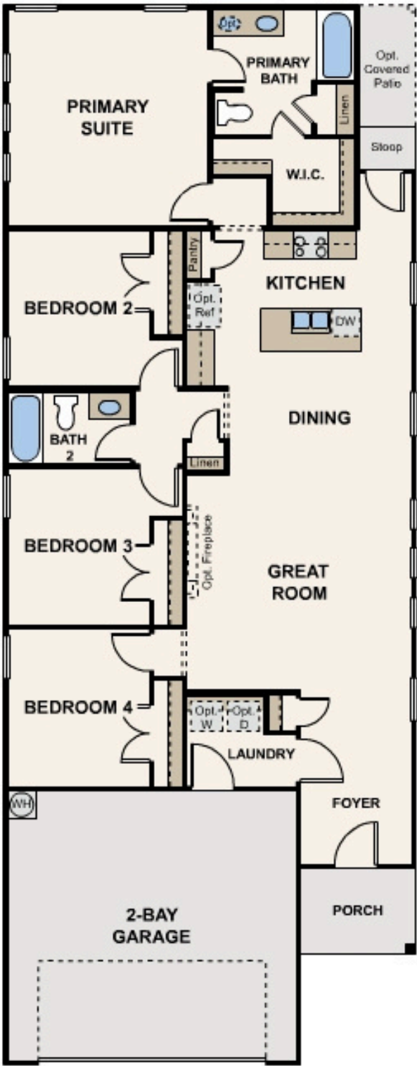
FLOOR PLAN
