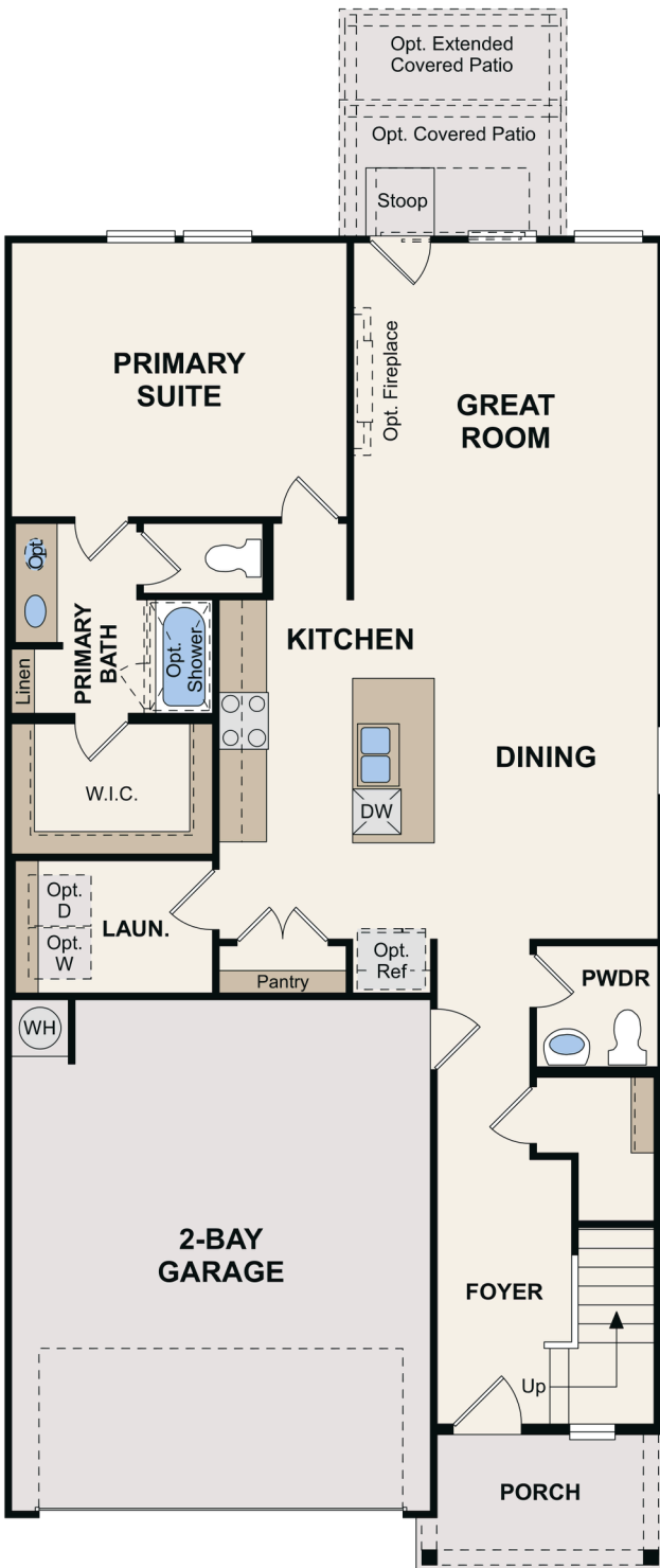
FIRST FLOOR
